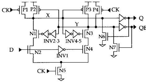
Fig. 7. Dual-rail dynamic flip-flop.
