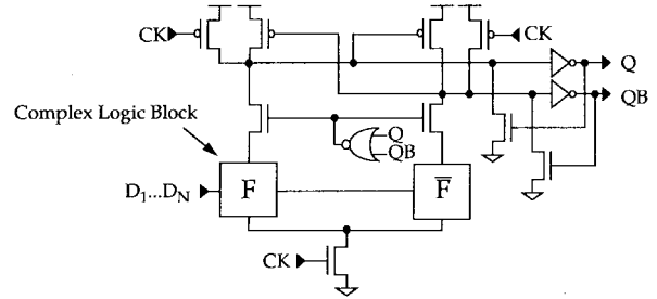
Fig. 8. Dual-rail DFF with embedded logic and common shutoff.
