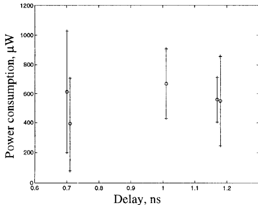
Figure 2. Power consumption versus delay for static flip-flops.
