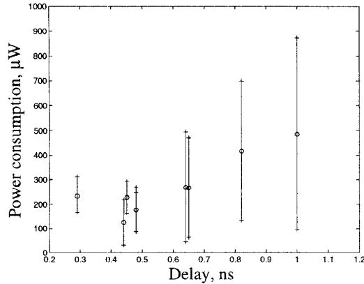
Figure 1. Power consumption versus delay for dynamic latches
