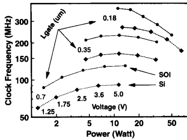
Fig. 16. Clock frequency versus power comparing Si and SOI technology for three generations. Higher speed at constant power or lower power at constant speed may be realized.
