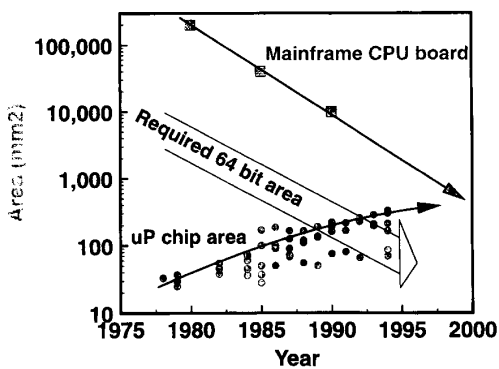
Fig. 2. Microprocessor chip area versus year as reported at ISSCC conferences. The trend is compared with the area required to implement a 64 b processor, and with an extrapolation of the mainframe board area.
