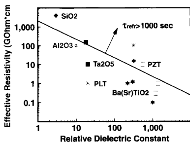
Fig. 13. Required dielectric resistivity and permittivity to determine the feasibility of new insulators for DRAM cell applications. Few examples meet these (minimum) criteria.
