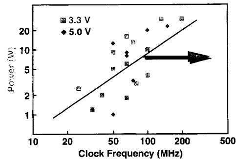
Fig. 4. Recent data reported on power versus frequency for microprocessors. Only a slight shift is observed due to the transition from 5 to 3.3 V supply voltage.
