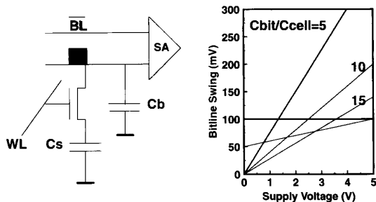
Fig. 12. Bitline voltage appearing to the sense amplifier decreases with reduced supply/plate voltage. The bitline capacitance needs to be scaled faster than the storage capacitor (adapted from [10]).
