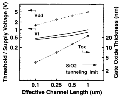
Fig. 14. The ratio between power supply and threshold voltage is decreasing for sub 0.25 \mu\text{m} devices. Gate oxide thickness is approaching fundamental tunneling current limits below 3 nm [14].
