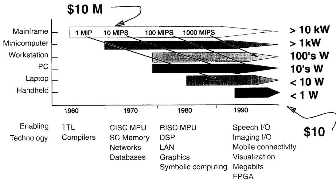
Fig. 1. Both power/MIPS and price/MIPS have decreased by orders of magnitude over the past two decades (adapted from [2]).
