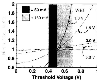
Fig. 15. Delay variations due to threshold voltage shift, assuming a constant worst-case V_t of 0.4 V. The delay sensitivity to becomes intolerable when V_t increases to more than 75% of V_{dd} (adapted from [10]).
