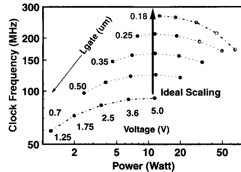
Fig. 7. Clock frequency versus power for various supply voltages and gate length dimensions. Maximum performance stays at about the same power per chip.
