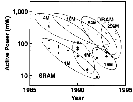
Fig. 10. Active power trends for DRAM and SRAM chips. Factors of 10 in power-per-bit have been achieved per generation for the DRAM. The power need for SRAM has stayed below DRAM until this time but is driven up by high speed requirements. (Adapted from [10]).
