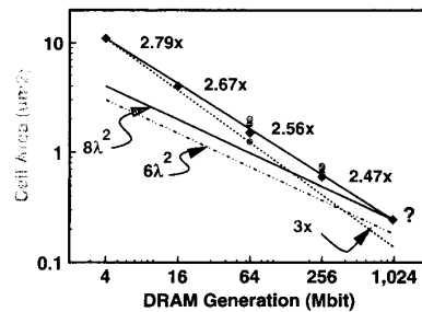
Fig. 11. DRAM cell area versus lithography generation. The extrapolated trends and requirement lines cross over at the 1 Gb generation, indicating vanishing design margins. Reducing cell area requirements to less than eight lithographic squares provides for continued scaling of the conventional transistor + capacitor cell.
