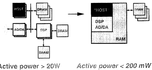
Fig. 3. A general speech recognition system is implemented with a general purpose micro-processor, a specialized DSP chip, SRAM as well as DRAM and EEPROM for memory, and also A/D and D/A functions. Scaled technology has the capability to integrate the whole system on one or two chips, if the various technology elements can be merged economically.
