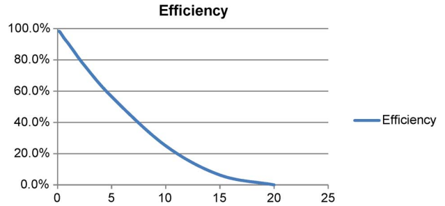
Fig. 9. Efficiency versus angle limited by fringing field effects.
