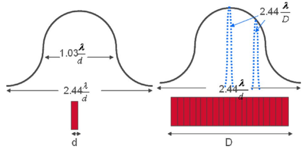
Fig. 2. The envelope under which beam steering occurs.
