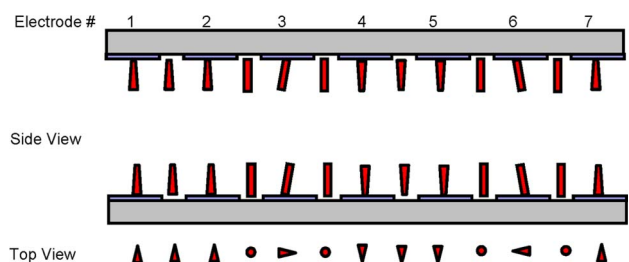
Fig. 25. V-COPA alignment setup.
