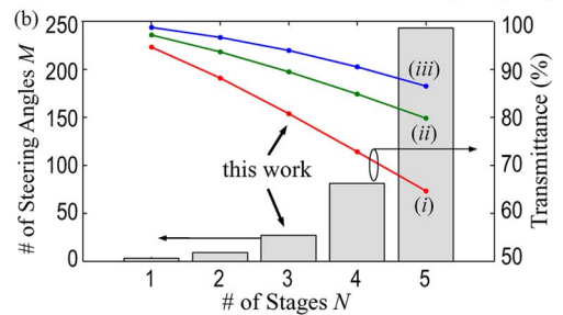
Fig. 2. (Color online) Ternary PG beam steering design: (a) three-stage ( N = 3 ) ternary steerer design has M = 27 discrete steering angles (only 9 illustrated, \Omega_l = \sin \theta_l ), (b) number of steering angles and calculated transmittance versus number of stages. Three cases of \{\eta_{\pm 1}, D, R, A\} in Eq. (5) are shown, as described in the text.
