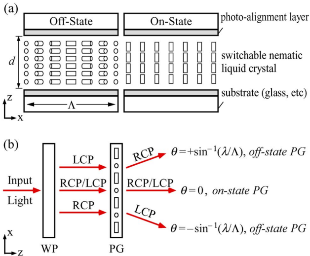
Fig. 1. (Color online) PG structure and single steering stage: (a) side view of a PG (on/off-state), showing LC director profile, (b) beam steering in single steering stage containing a WP and a PG, having different diffraction behavior with RCP and LCP incident light.
