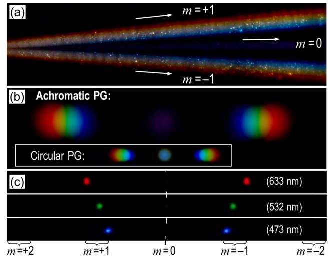
Fig. 3. (Color online) Photographs of achromatic PG diffraction. Unpolarized white LED light as seen from (a) plan view (intersecting a white card) and (b) projected screen view. (c) Linearly polarized laser light ( \Lambda = 6.5 \mu\text{m} ).
