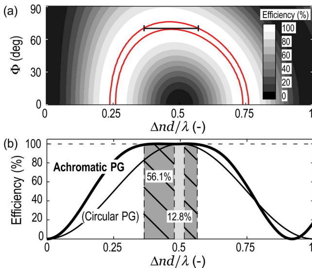
Fig. 2. (Color online) Theoretical diffraction of the achromatic PG. (a) First-order efficiency spectra versus twist angle \Phi ( \Sigma \eta_{\pm 1} \geq 99\% , outlined region). (b) First-order efficiency spectrum for \Phi = 70^\circ compared with the circular PG.
