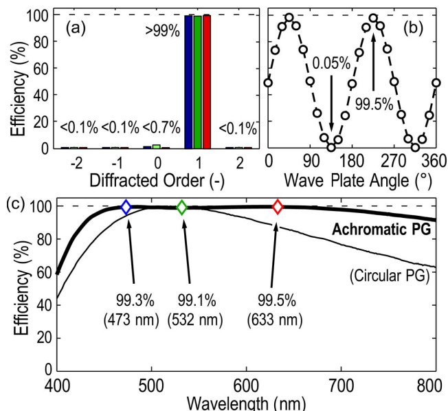
Fig. 4. (Color online) Measured diffraction of the achromatic PG. (a) Efficiencies with circularly polarized incident laser light [same wavelengths as in Fig. 3(c)]. (b) Polarization sensitivity of the m=+1 order with a rotating quarter-wave plate. (c) First-order efficiency spectrum from spectrometer (curves) and laser (diamonds) measurements.
