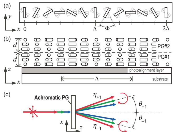
Fig. 1. (Color online) Achromatic PG. Nematic director profile (a) plan view and (b) side view. (c) Diffraction geometry (note only the m = \pm 1 orders emerge).
